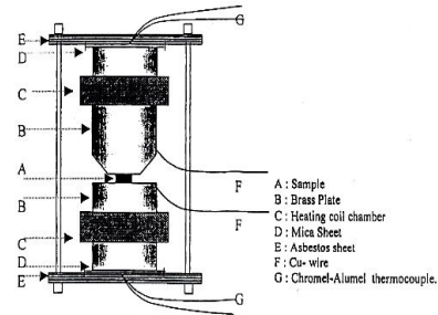
Fig. 2 Sample holder used for measurement of TEP.
