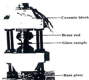
Fig. 1 : The sample holder used for ac/dc and transference number measurements of silver borate glass.
